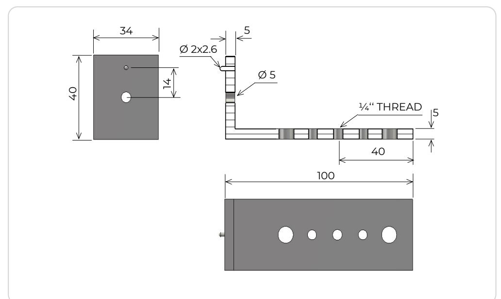
Mounting flange
