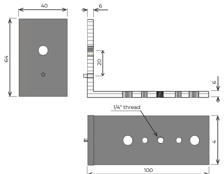
Mounting flange
